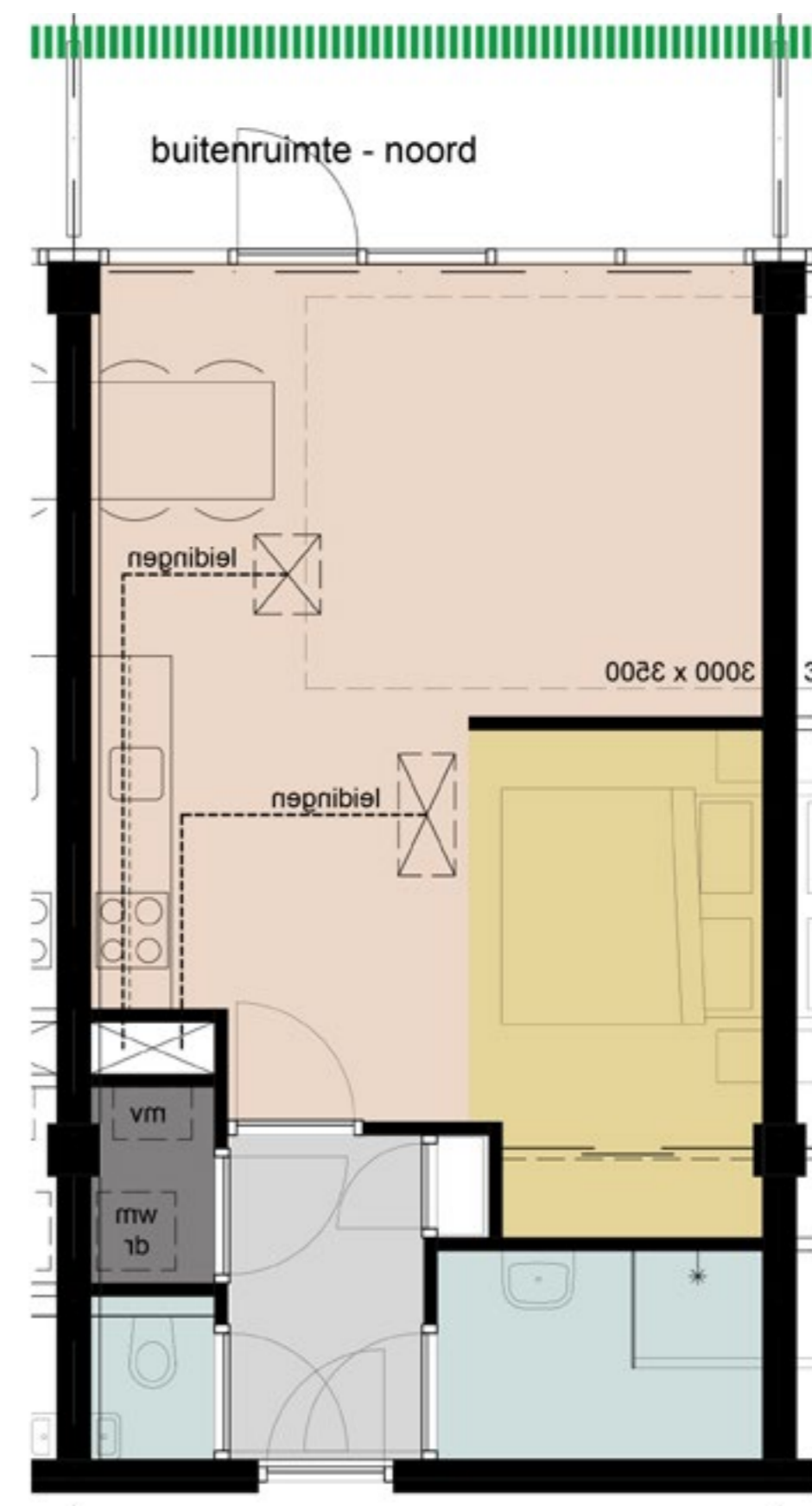
Plattegrond studio
